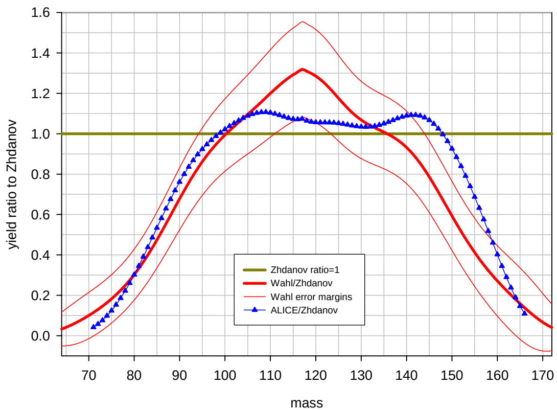
Benchmark B: ^{237}\text{Np} at 50 MeV, pre-neutron emission yield ratio to Zhdanov's data
